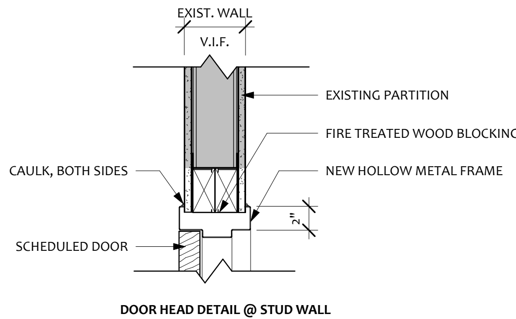
2 TYP. HM FRAME AT EXIST. WALL 1 1/2" = 1'-0"
