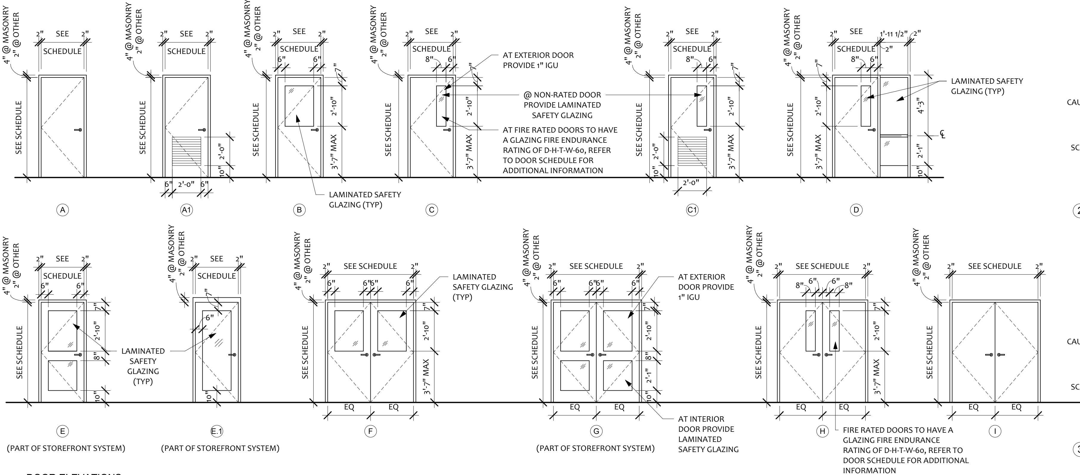
1 DOOR ELEVATIONS 1/4" = 1'-0"
